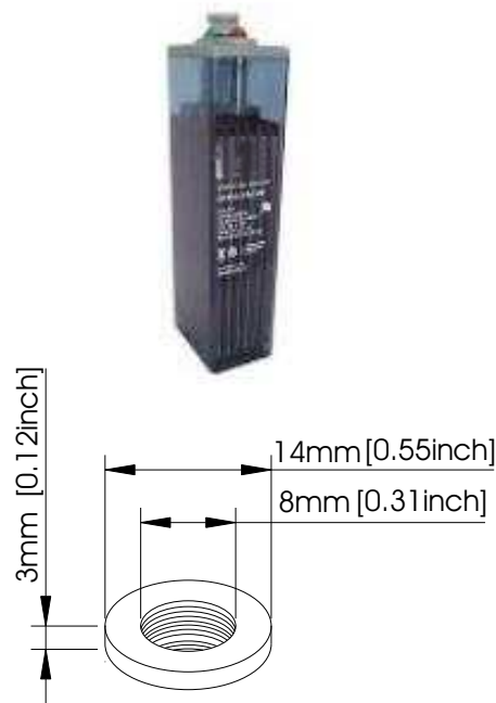
Terminal Dimensions
