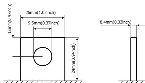
Terminal Dimensions
