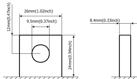
Terminal Dimensions
