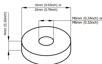
Terminal Dimensions
