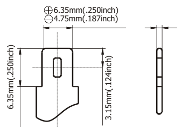
Terminal Dimensions
