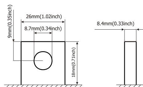
Terminal Dimensions
