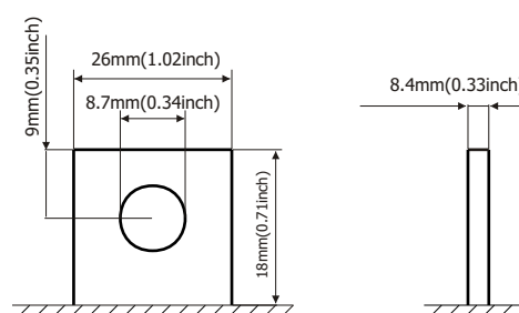
Terminal Dimensions
