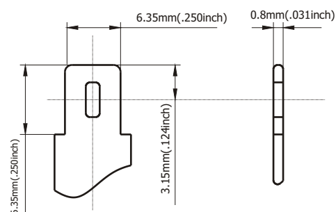
Terminal Dimensions
