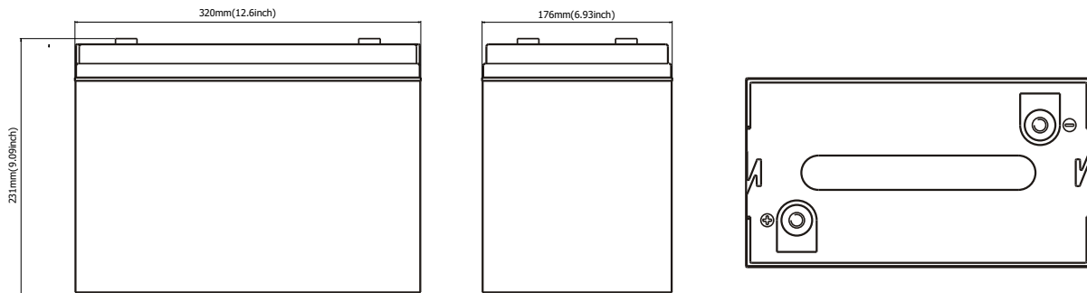
Terminal Dimensions
